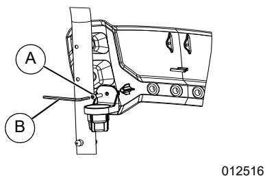
Figure 2-3. Porte-buse accessoire
