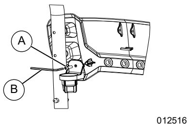
Figure 2-3. Accessory Nozzle Holder
