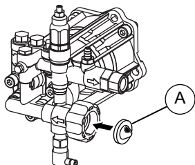
Figure 2-11. Inspect Inlet Screen
