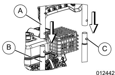
Figure 2-1. Enfiler le guidon
