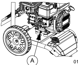
Figure 4-7. Oil Drain Plug
