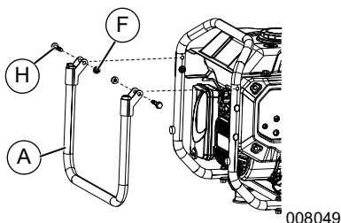
Figure 2-11. Handle Assembly
