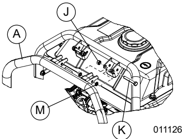
Figure 2-11. Handle Assembly
