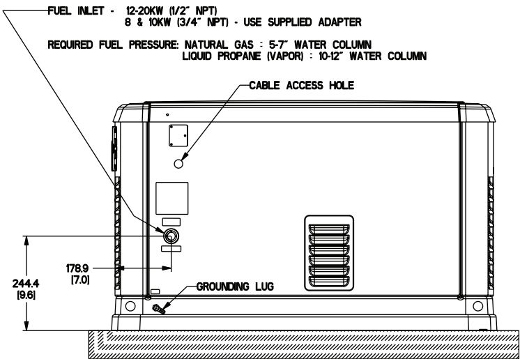
REAR VIEW
