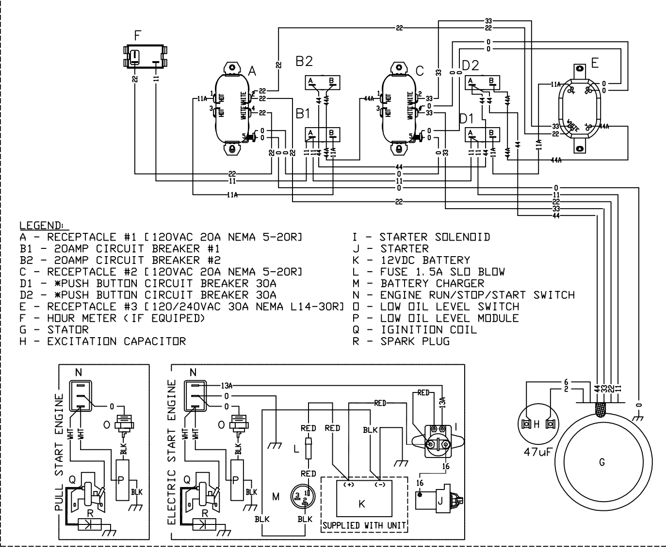
WIRING - DIAGRAM
