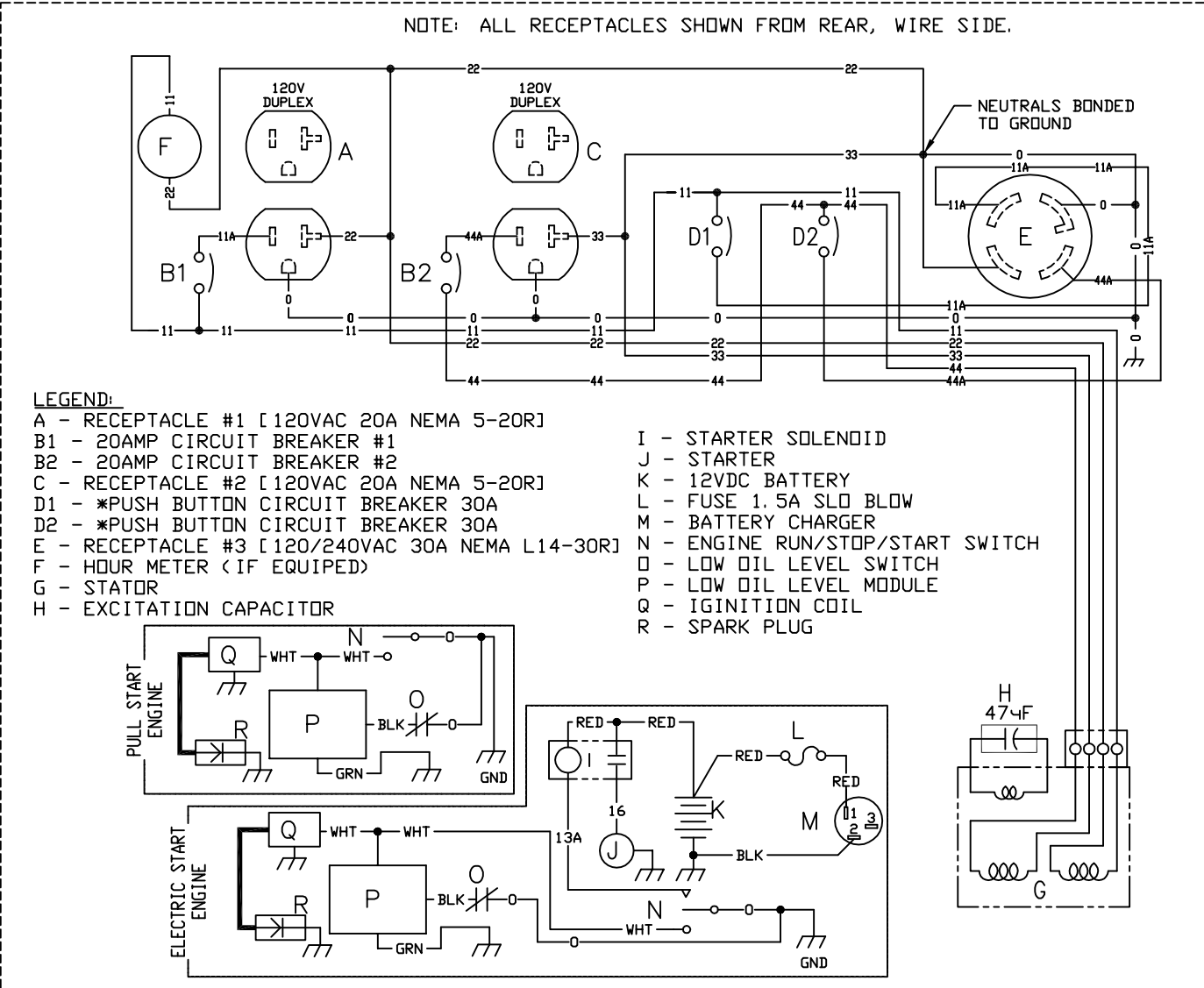
SCHEMATIC - DIAGRAM
