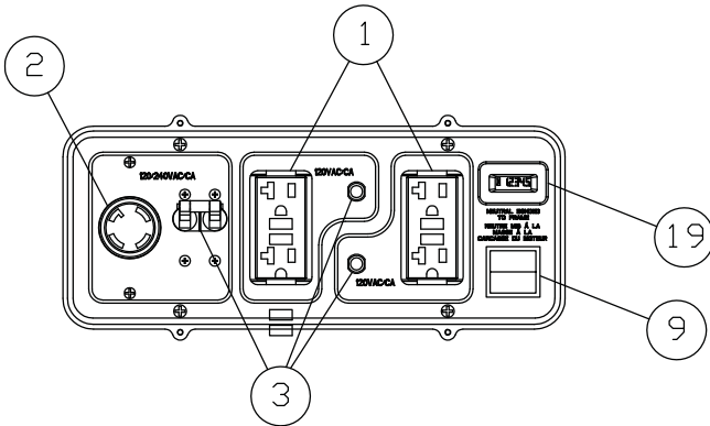
Figure 2C - Control Panel (CSA Models)
