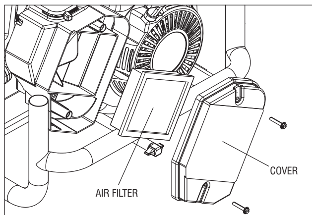
Figure 13 – Air Filter
