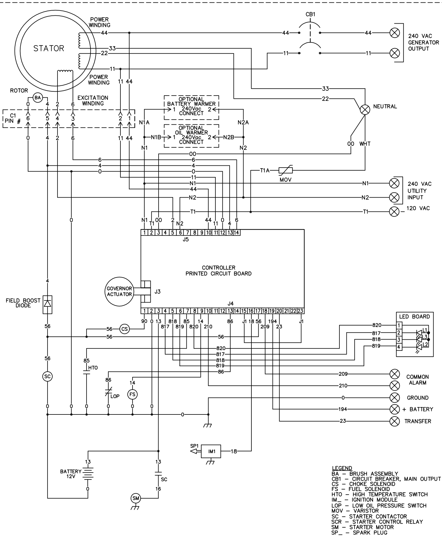
SCHEMATIC - DIAGRAM
