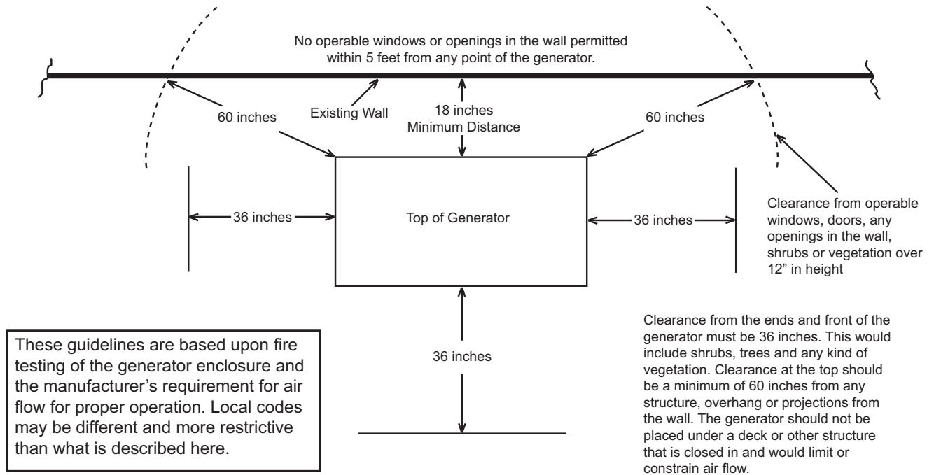
Figure 1.10 – Installation Guidelines
