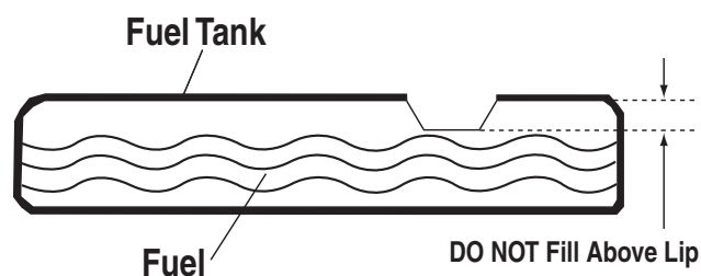
Figure 9 - Fuel Tank
