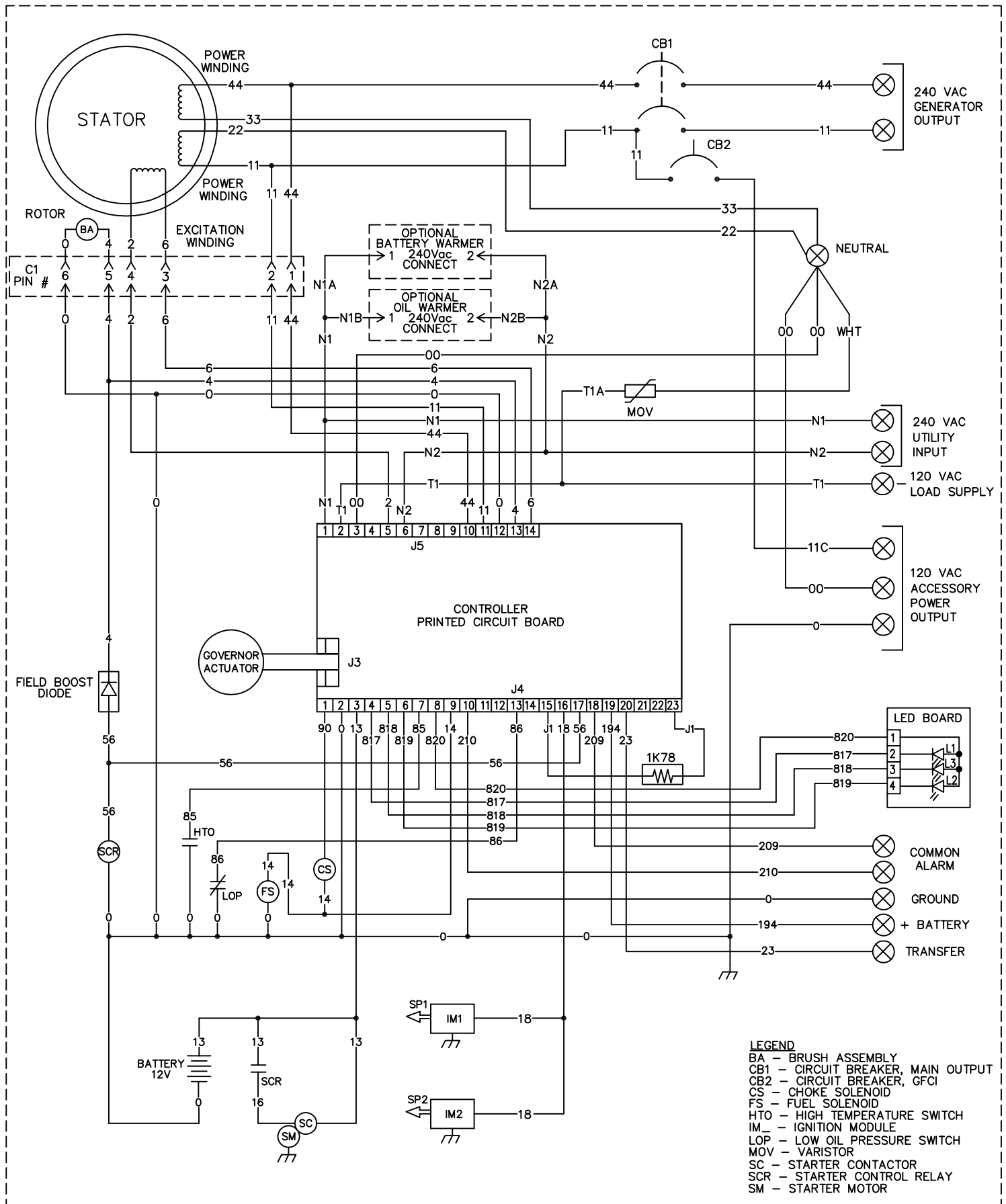
SCHEMATIC - DIAGRAM
