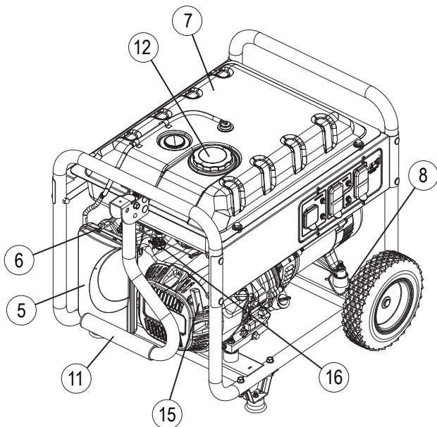
Figure 3A - Generator Controls (GP5000/GP6000)
