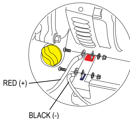
Figure 15 - Battery Connections
