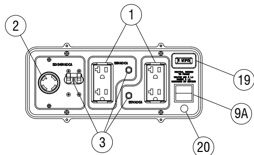
Figure 3 - Generator Controls
