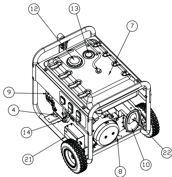
Figure 4 - Generator Controls
