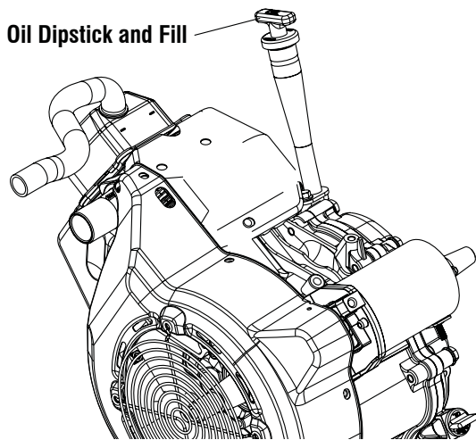
Figure 4.2 — Oil Dipstick, 10kW
