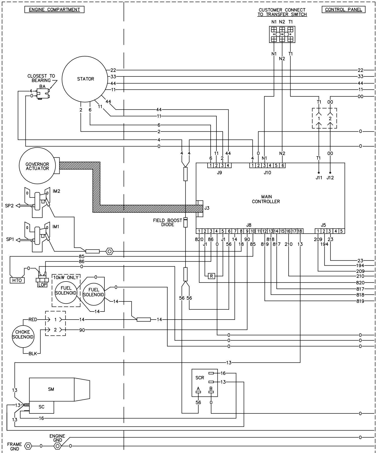
WIRING - DIAGRAM
