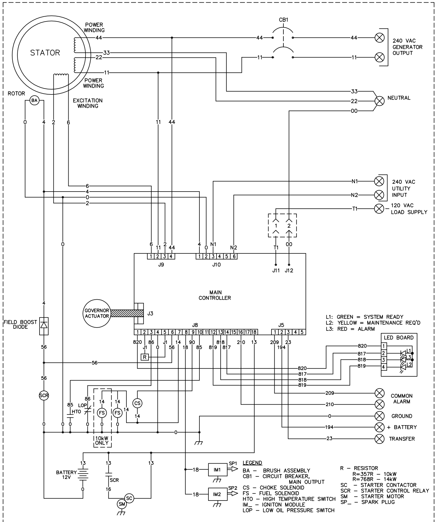
SCHEMATIC - DIAGRAM
