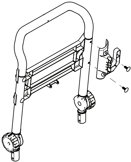
Figure 2 – Attach Gun Hook to Handle Assembly
