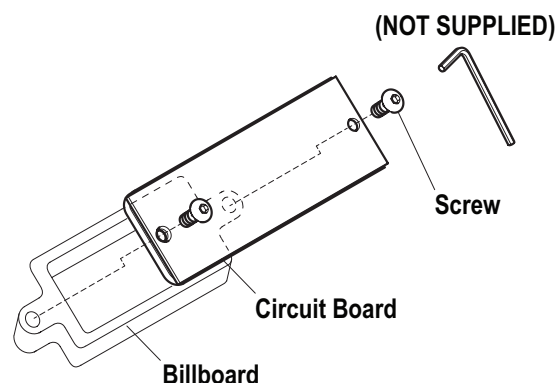
Figure 32 – Circuit Board
