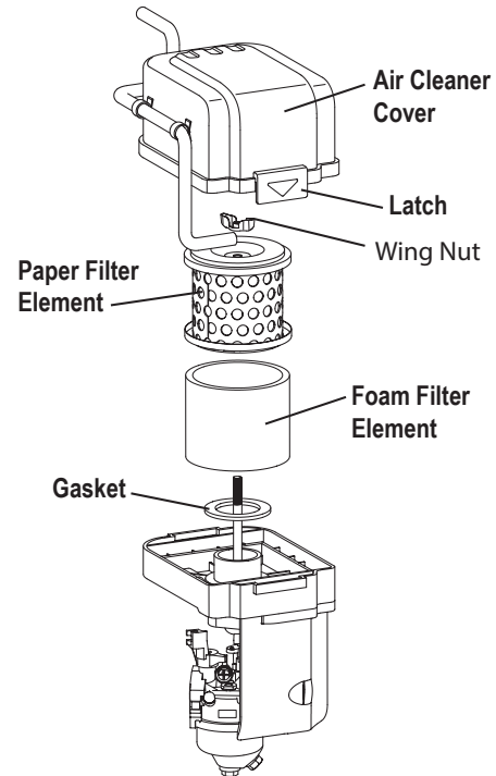
Figure 41 – Service the Air Cleaner
