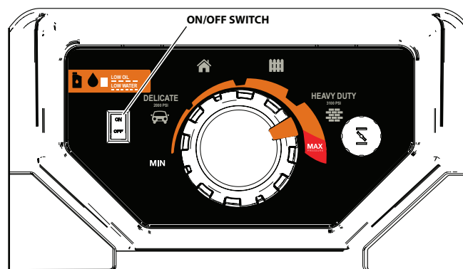
Figure 26 – ON/OFF Switch
