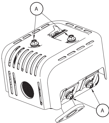
Figure 44 – Retirer le pare-étincelles
