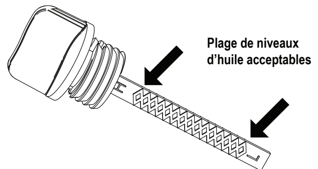
Figure 39 – Jauge
