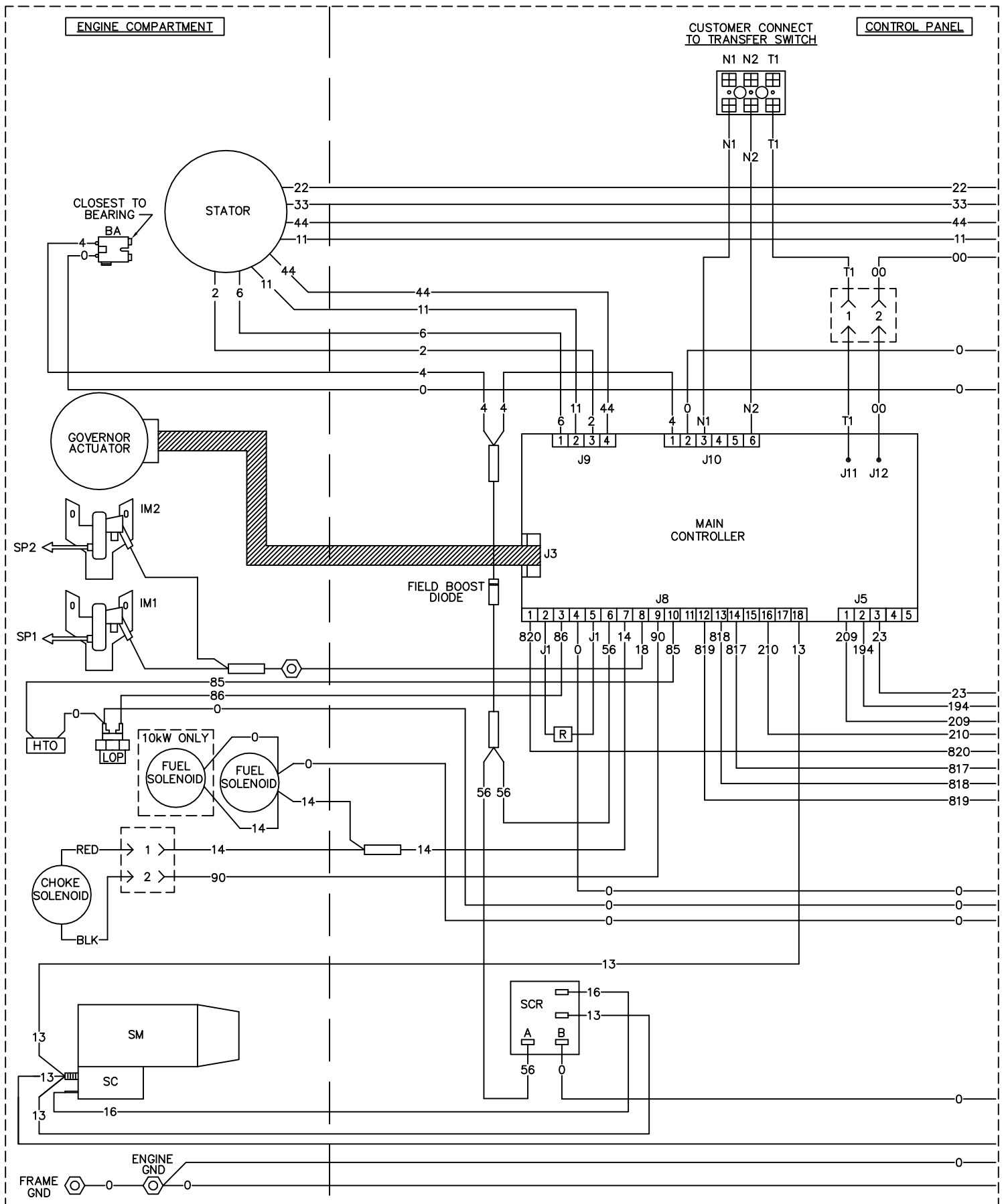
WIRING - DIAGRAM
