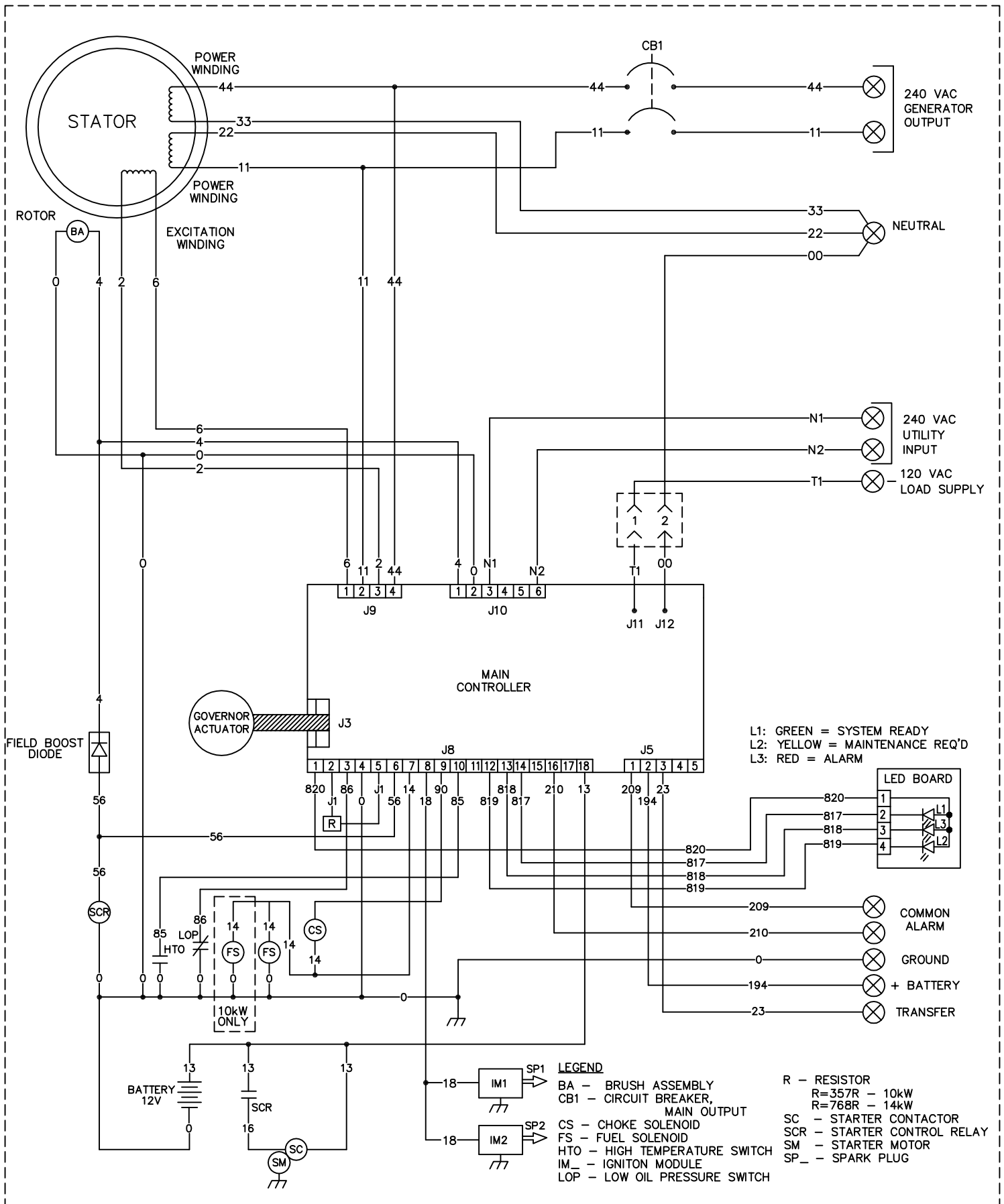
SCHEMATIC - DIAGRAM
