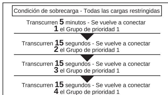
Figure 2.2 - Standard Load Shed
