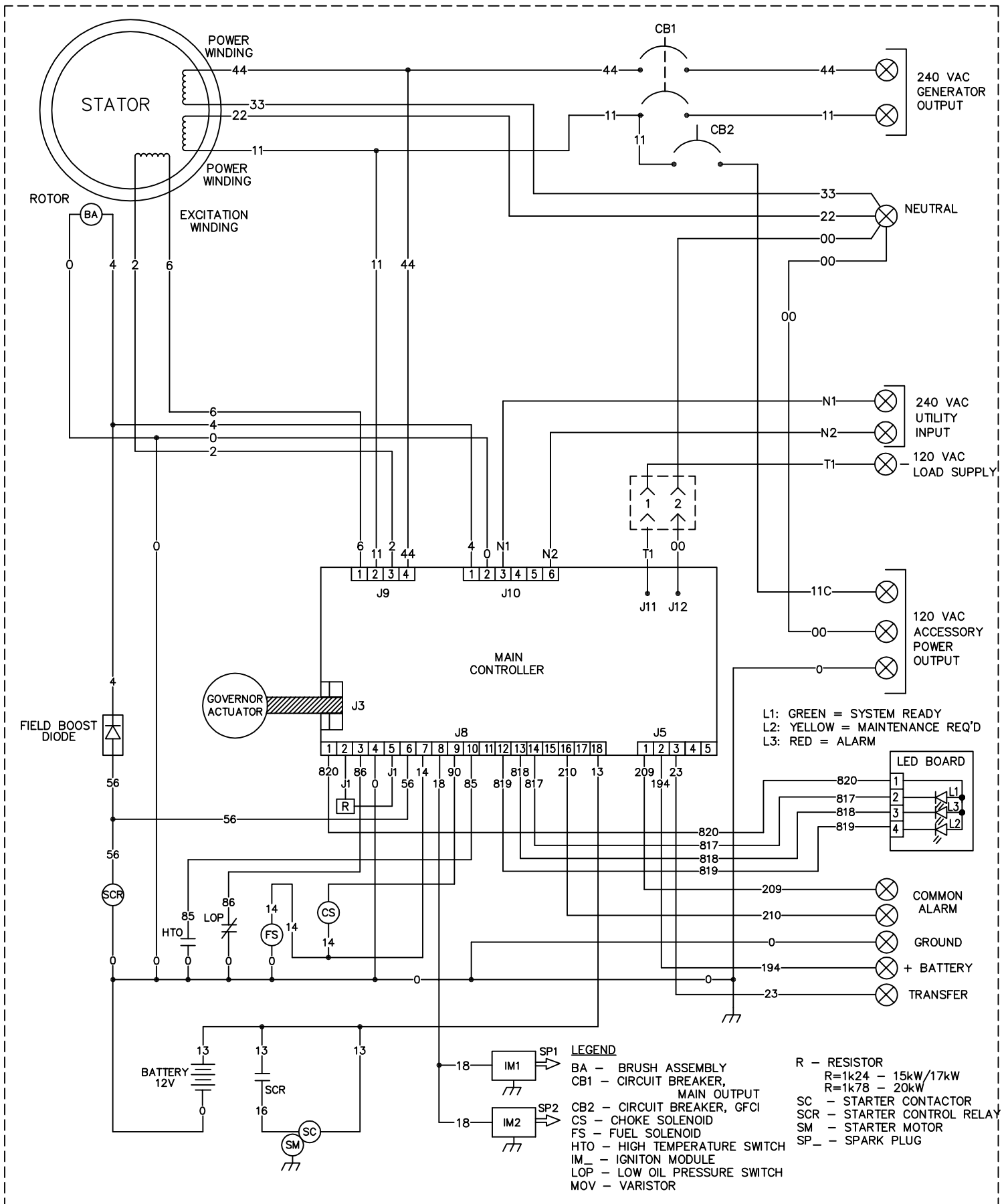
SCHEMATIC - DIAGRAM
