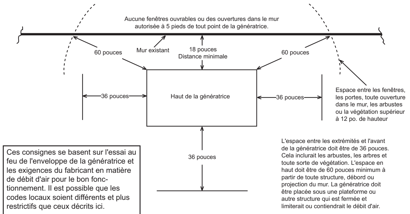
Figure 1.10 – Directives d'installation
