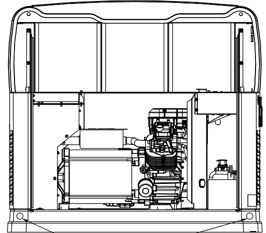
Ø30.2 Ø1.27 LIFTING HOLES 4 CORNERS
