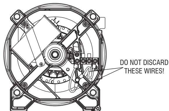
NEUTRAL TO FRAME GROUND XG7000 & 8000 BRUSHLESS ALTERNATOR ONLY
