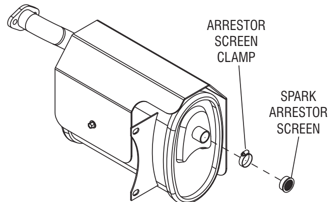
Figure 15 – Spark Arrestor Screen
