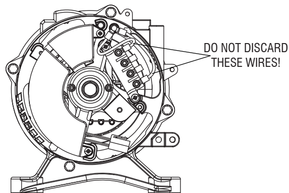
NEUTRAL TO FRAME GROUND XG6500, 7000 AND 8000 BRUSHED ALTERNATOR
