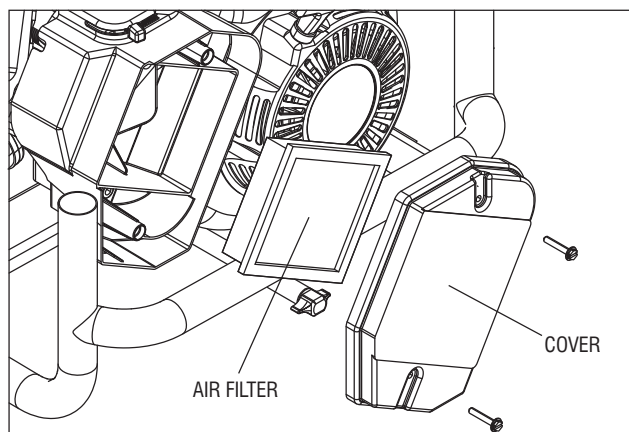
Figure 13 – Air Filter
