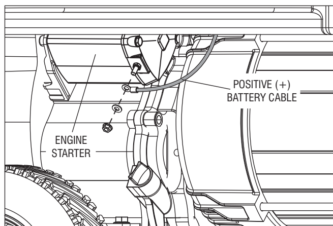
Figure 4 – Battery Connection
