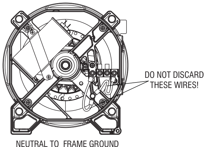
Figure 7 – Neutral to Frame Ground
