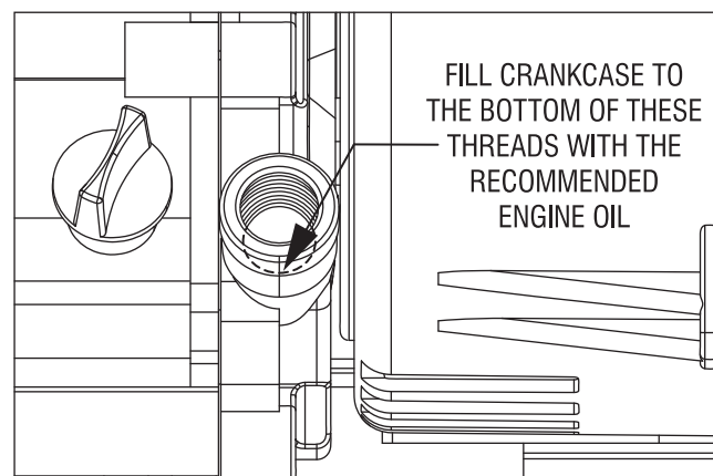
Figure 8 – Oil Level
