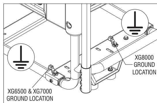
Figure 6 – Generator Ground Location
