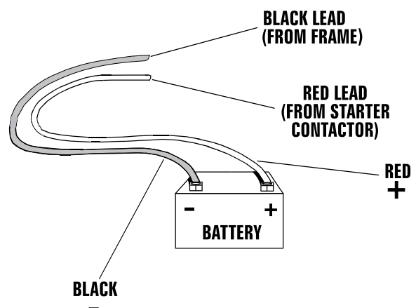
Figure 1.9 – Battery Cable Connections
