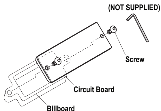
Figure 32 – Circuit Board
