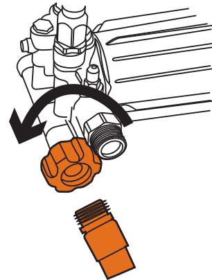
Figure 12 – Connect Garden Hose
