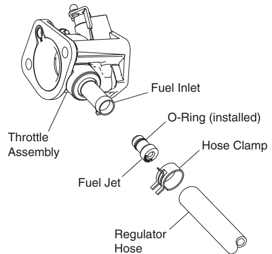
Figure 1.5 — Remove Fuel Jet
