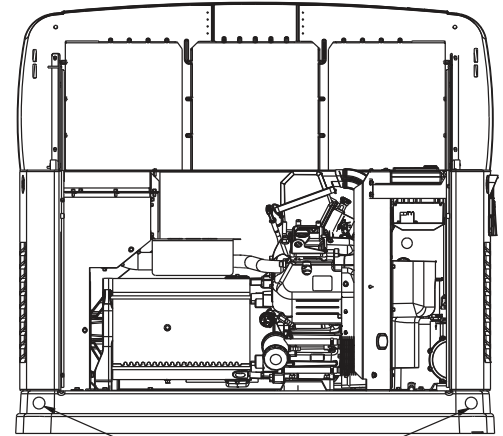
LIFTING HOLES 4 CORNERS Ø 30.2 [Ø 1.2]
