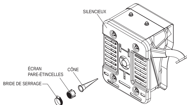
Figure 16 – Pare-étincelles
