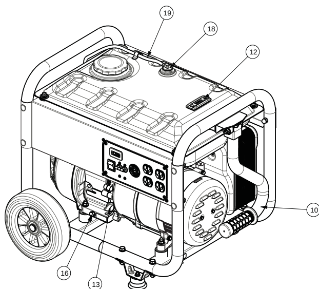
Figure 5 - Generator Controls
