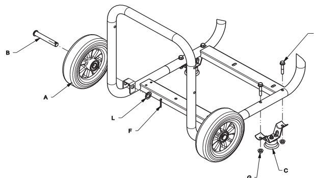
Figure 1 – Wheel Assembly
