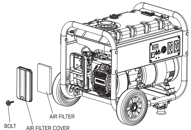
Figure 17 - Air Filter
