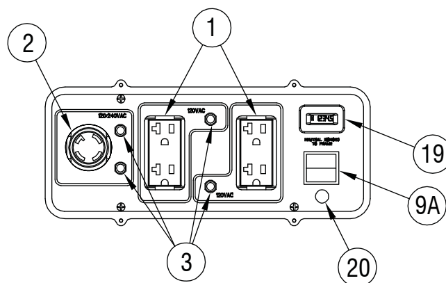
Figure 2A - Control Panel (49 State Models)
