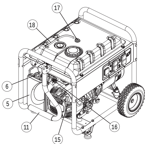
Figure 4 - Generator Controls
