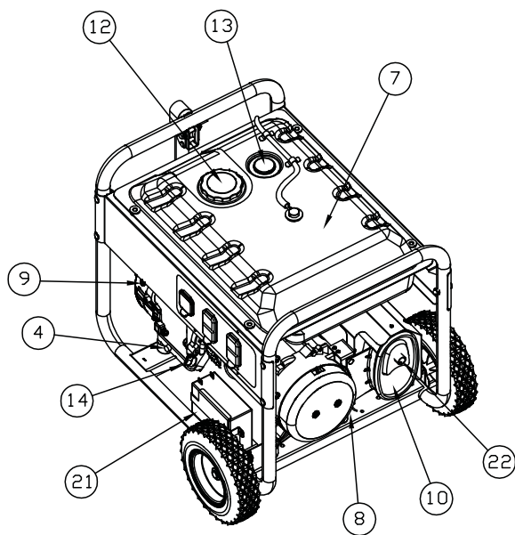
Figure 4 - Generator Controls
