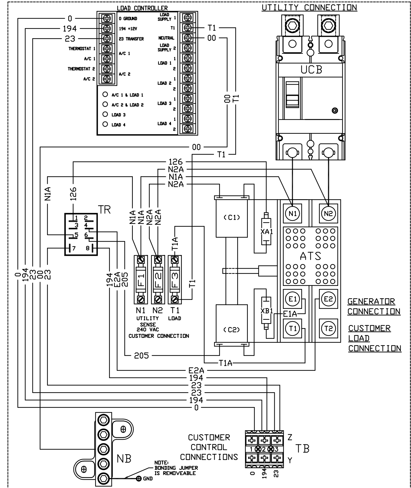
WIRING – DIAGRAM
