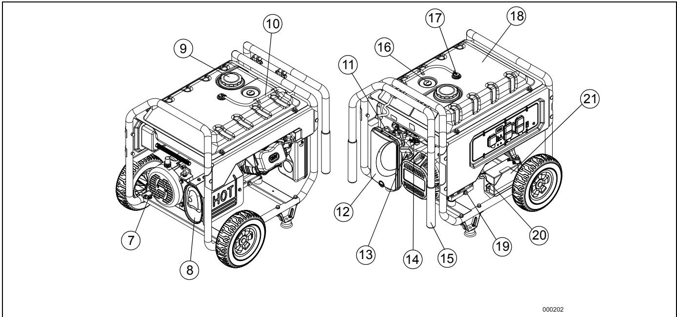
Figure 2-6. Generator Controls
