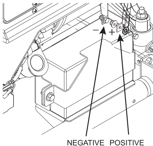
Figure 2-4. Battery Connections
