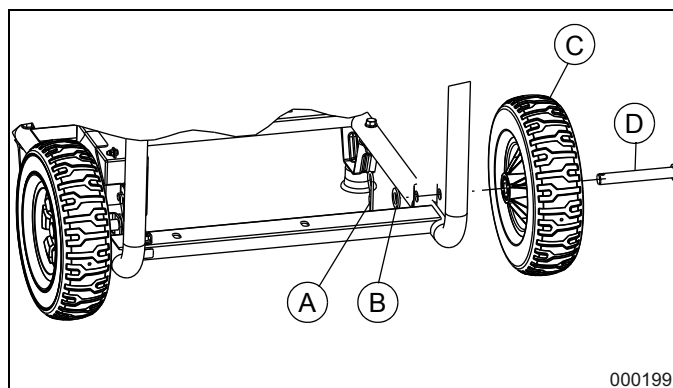
Figure 2-1. Ensemble de roue
