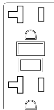
Figure 2-8. Prise duplex DDFT de 120 V c.a., 20 A
