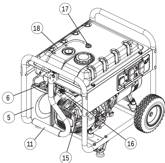
Figure 4 - Generator Controls
