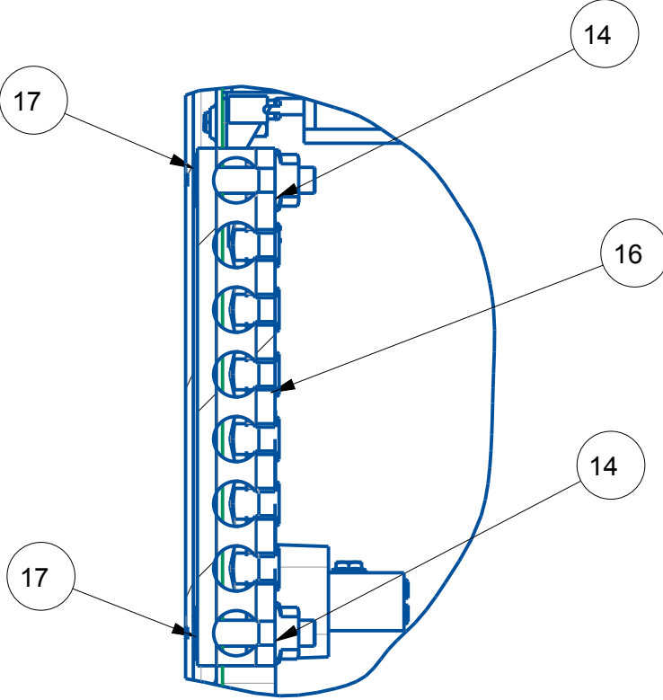
SECTION B-B SCALE 0.600
