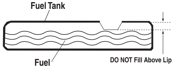
Figure 11 - Fuel Tank
