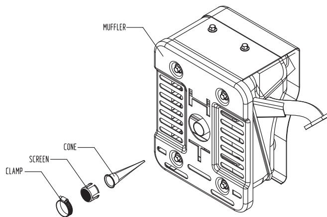
Figure 16 - Spark Arrestor
