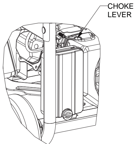
Figure 13 - Engine Controls
