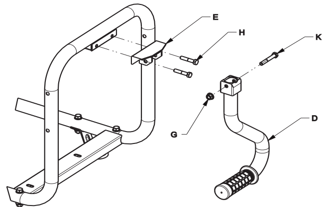
Figure 2 – Handle Kit
