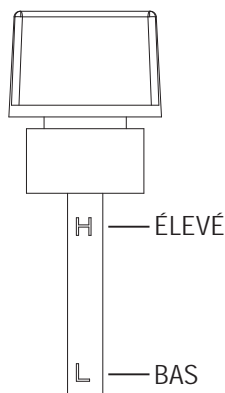
Figure 10 – Jauge
