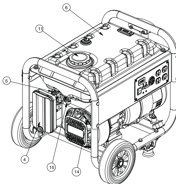
Figure 4 - Generator Controls
