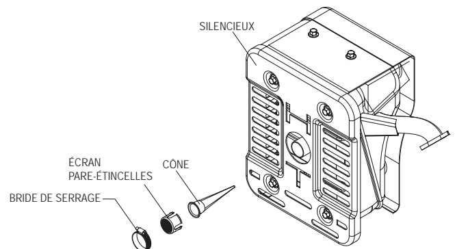
Figure 16 – Pare-étincelles
