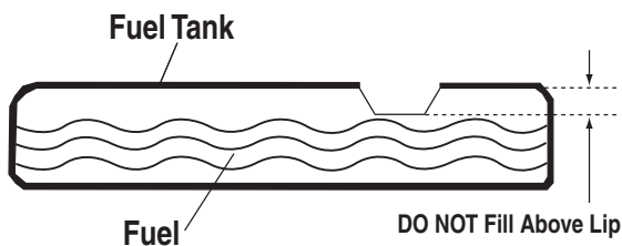
Figure 11 - Fuel Tank
