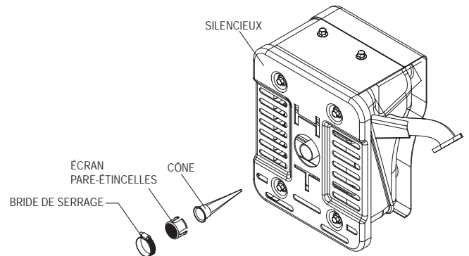
Figure 16 – Pare-étincelles
