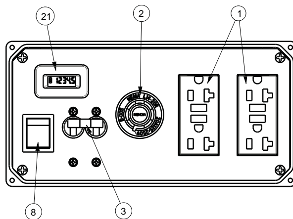
Figure 4 - Generator Controls
