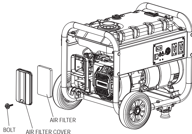
Figure 17 - Air Filter
