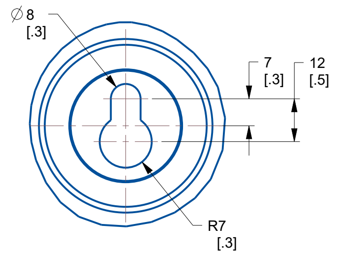
DETAIL A SCALE 1.000
