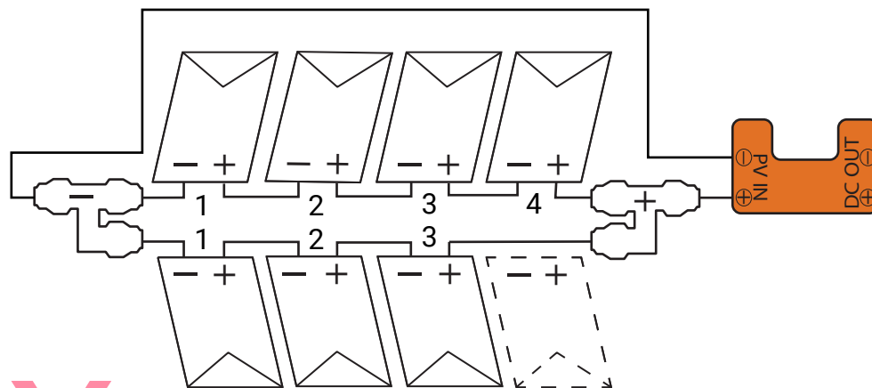
Parallel substrings must have same number of PV modules
