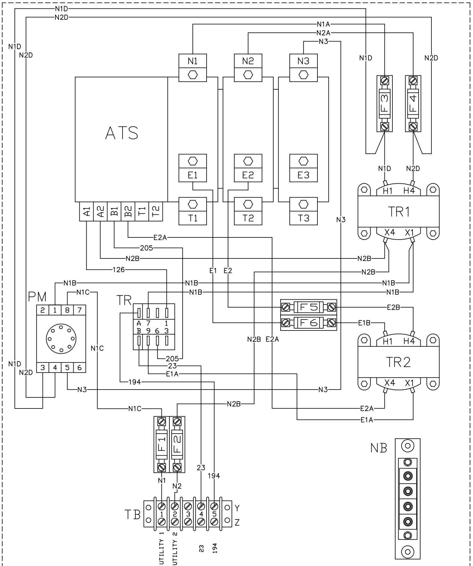
WIRING - DIAGRAM 400 AMP 480VAC DRAWING #: 0J1777
