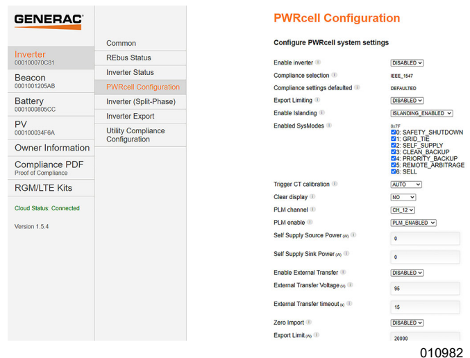
Figure 6-29. Configuration PWRcell
