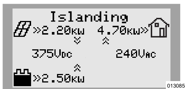
Figure 7-28. Mode îlotage
